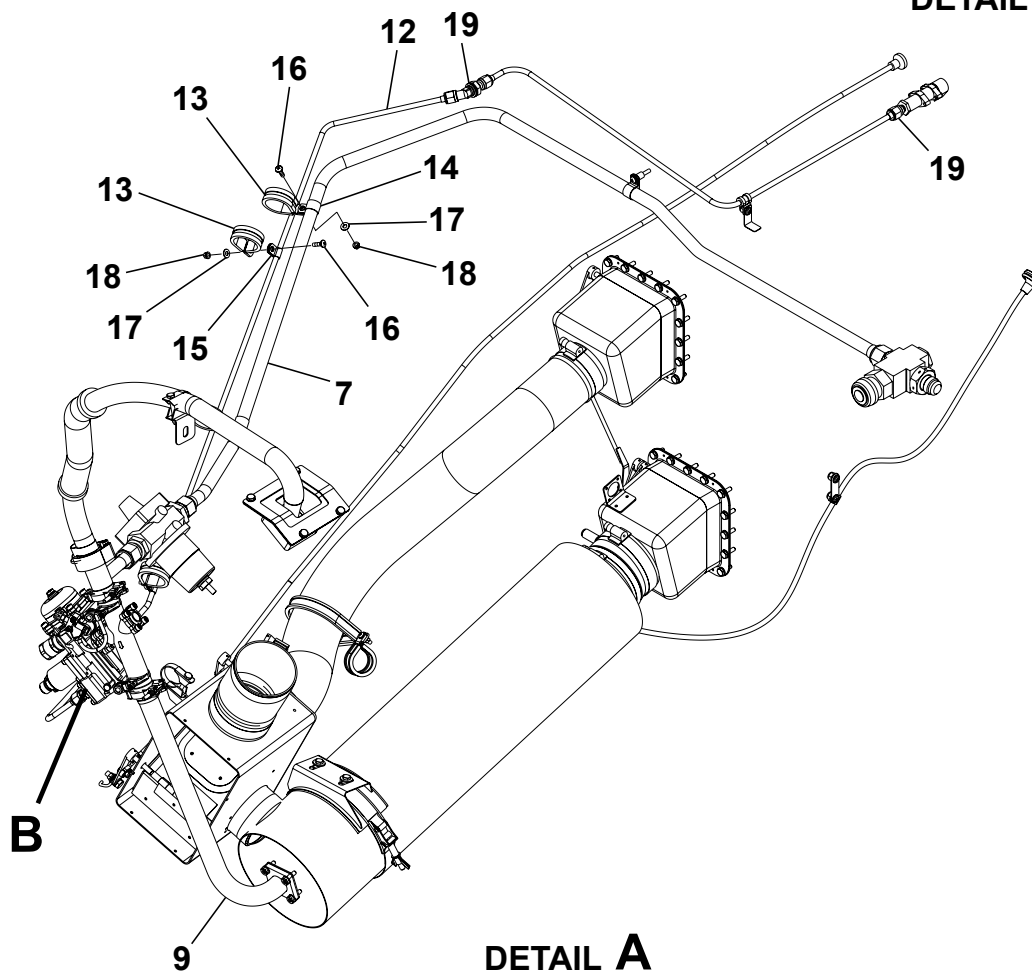
FLOW CONTROL VALVE INSTALLATION Figure 03. (Sheet 1)
