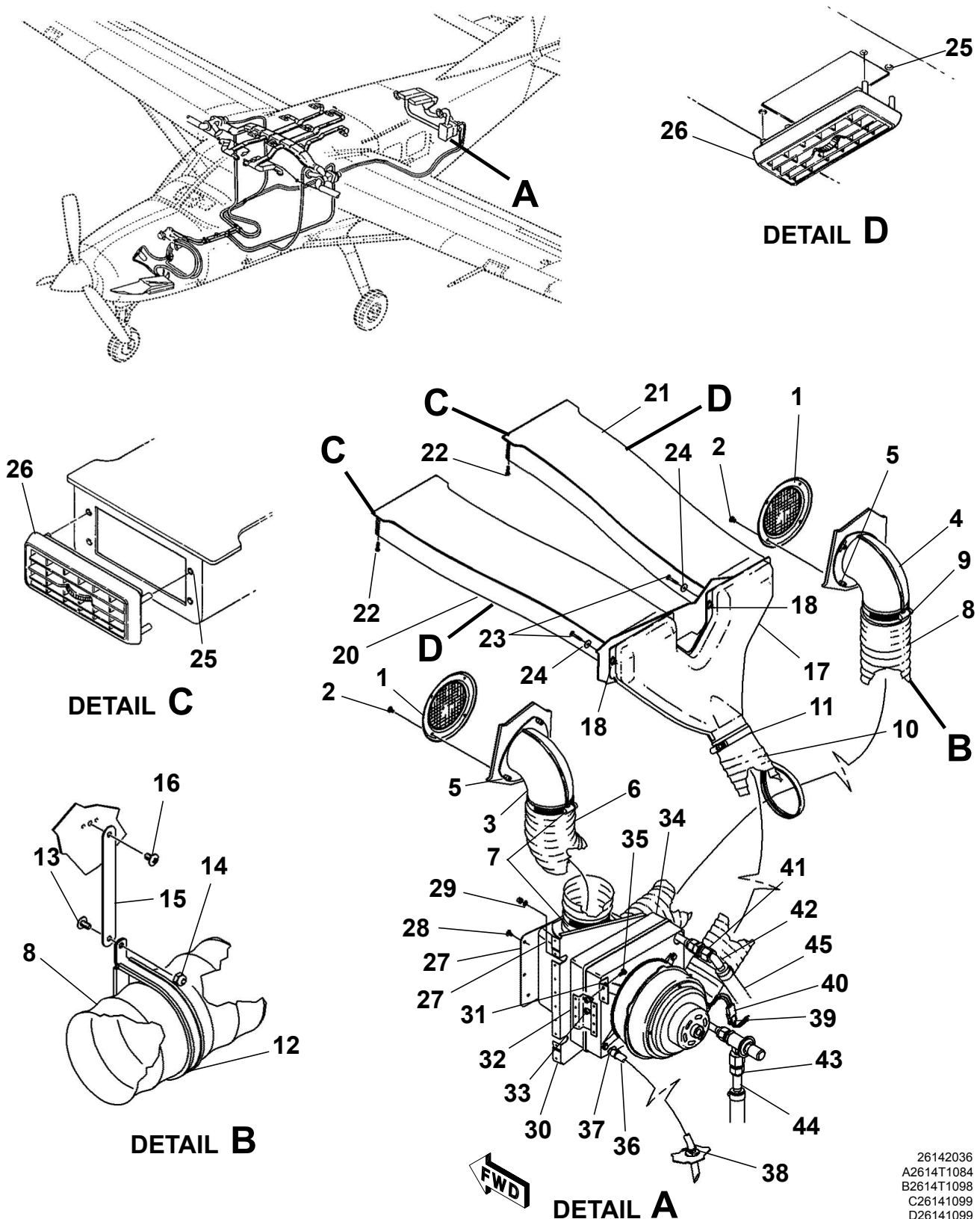
EVAPORATOR INSTALLATION - AFT MOUNTED Figure 02. (Sheet 1)
