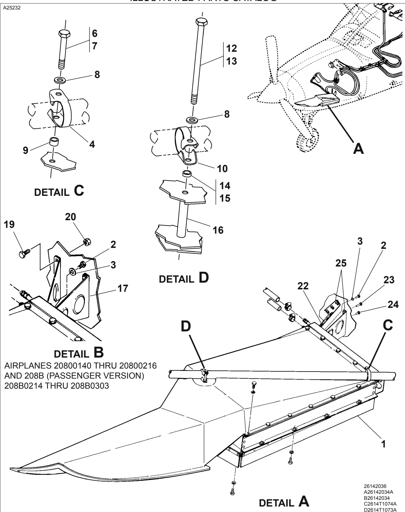
AIR CONDITIONER CONDENSER INSTALLATION Figure 01. (Sheet 1)
