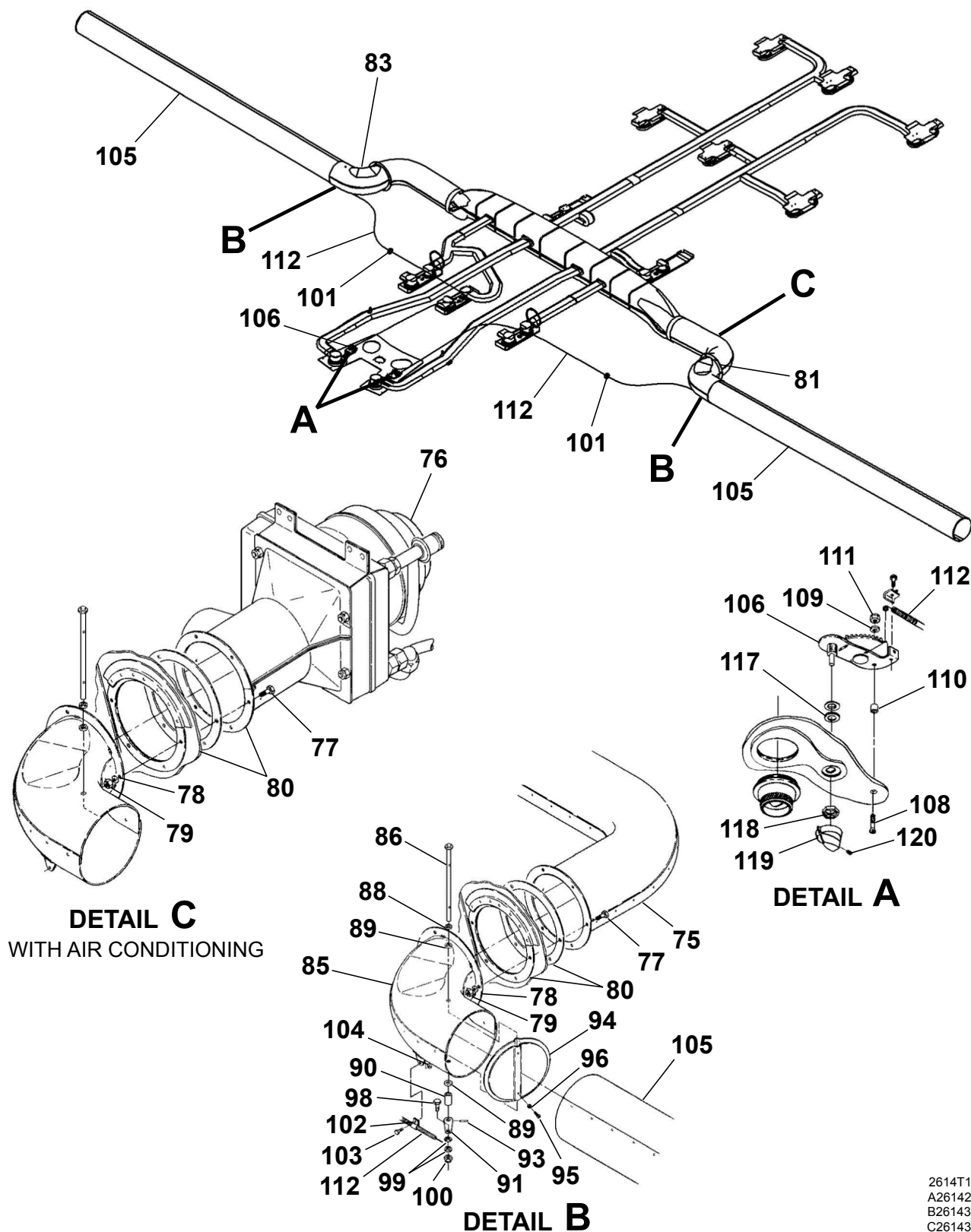
OVERHEAD VENTILATION SYSTEM PASSENGER VERSION Figure 02. (Sheet 2)
