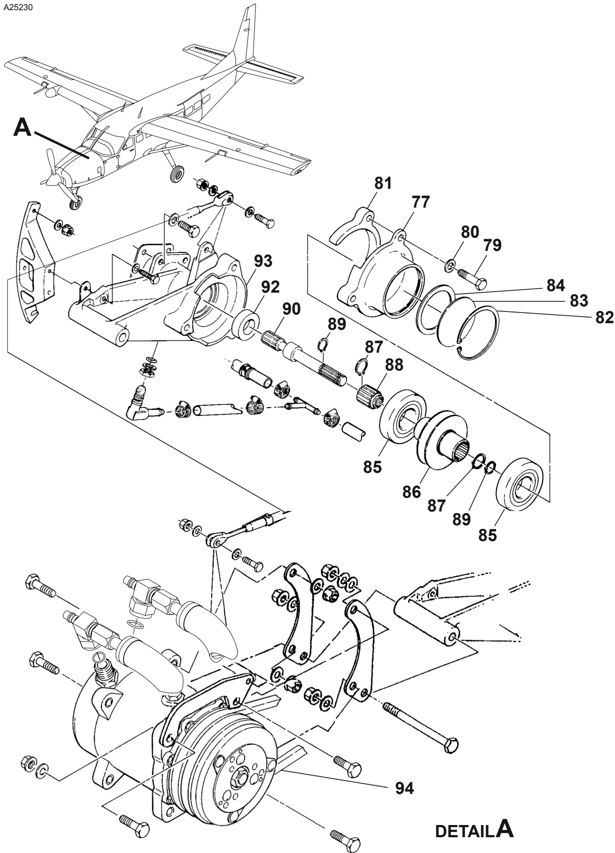
AIR CONDITIONER COMPRESSOR AND DRIVE UNIT INSTALLATION Figure 01. (Sheet 2)
