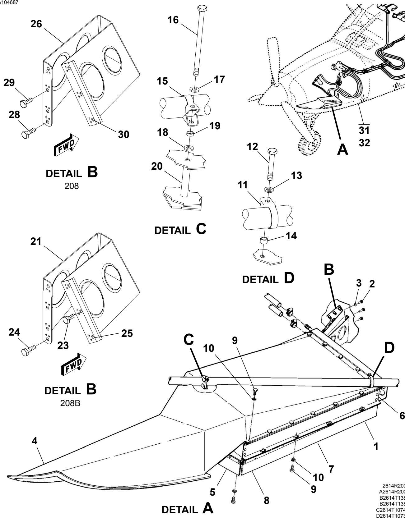
AIR CONDITIONER CONDENSER INSTALLATION Figure 01B. (Sheet 1)
