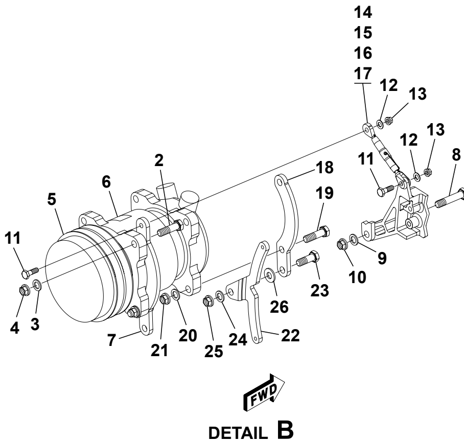
AIR CONDITIONER COMPRESSOR AND DRIVE UNIT INSTALLATION Figure 02. (Sheet 1)
