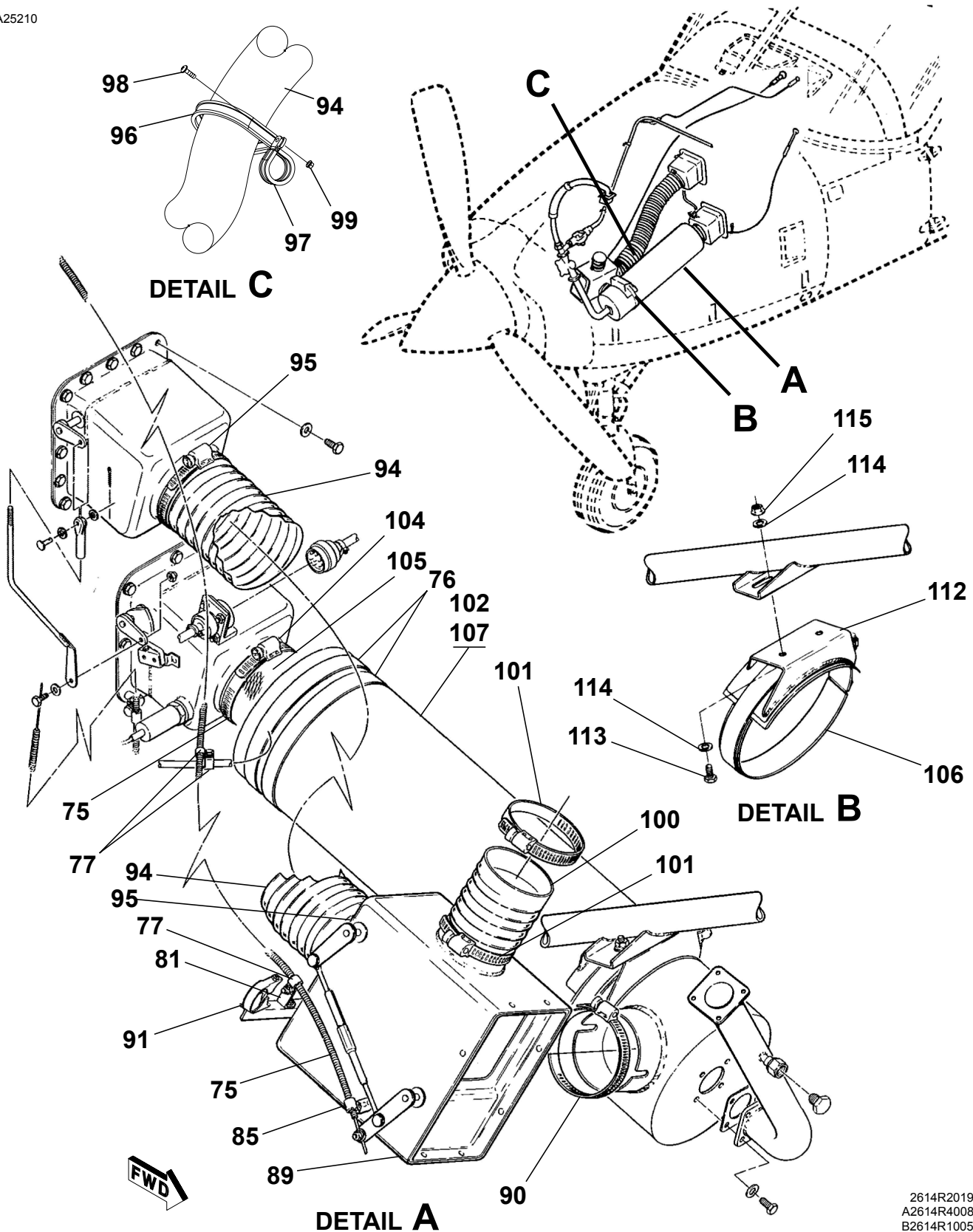
BLEED AIR HEATER COMPONENTS Figure 01. (Sheet 2)
