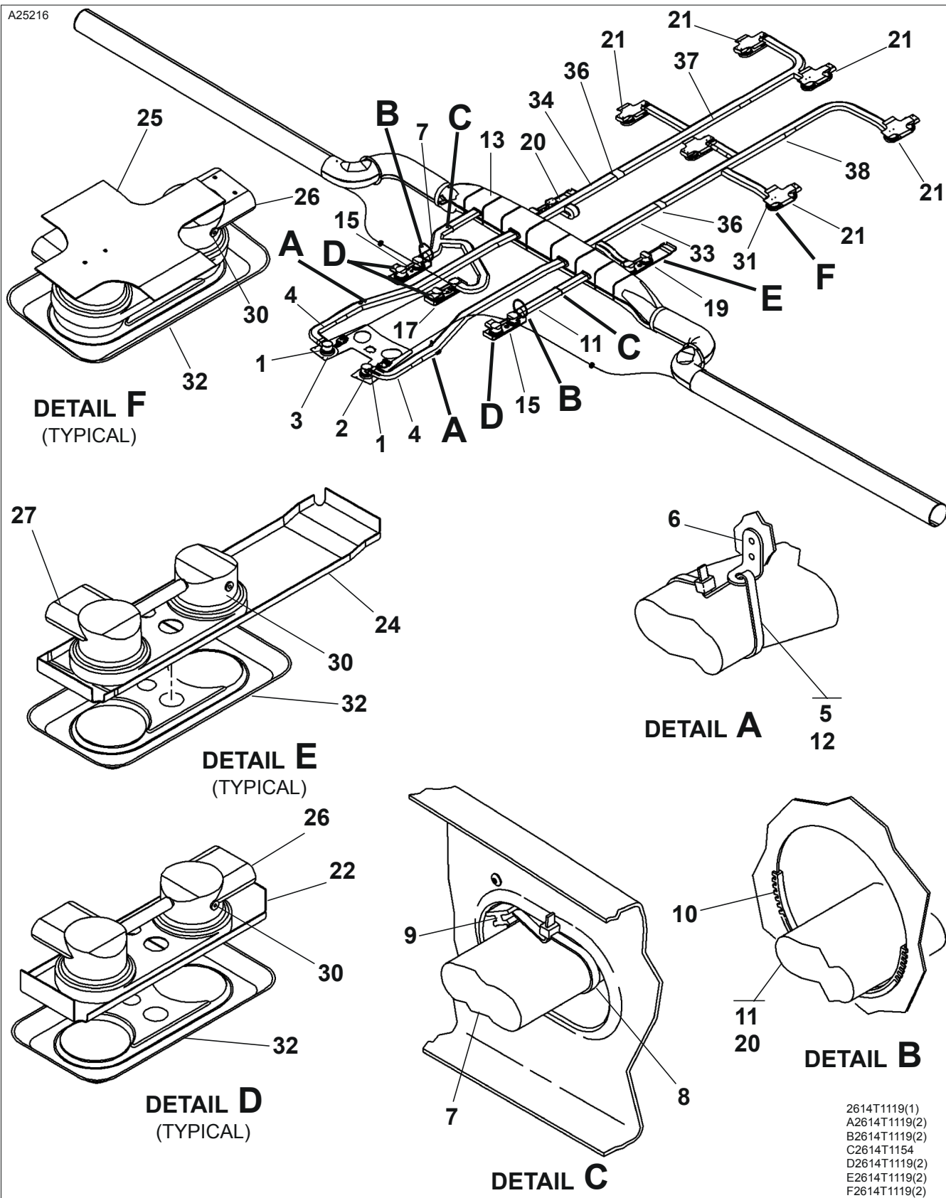
OVERHEAD VENTILATION SYSTEM PASSENGER VERSION Figure 02. (Sheet 1)
