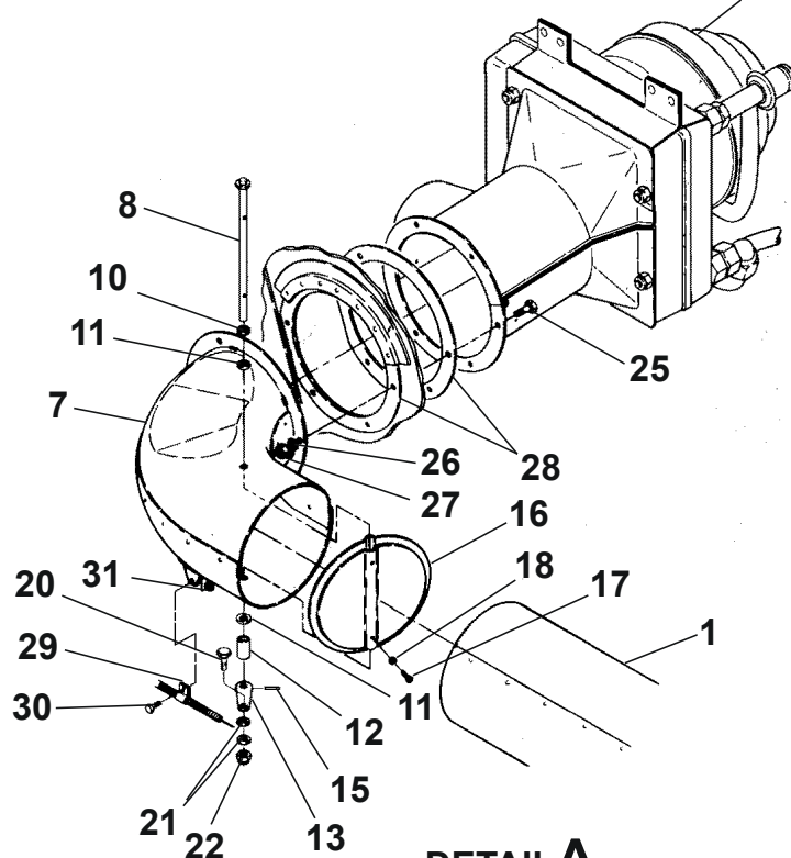
OVERHEAD VENTILATION SYSTEM WITH AIR CONDITIONING Figure 03. (Sheet 1)
