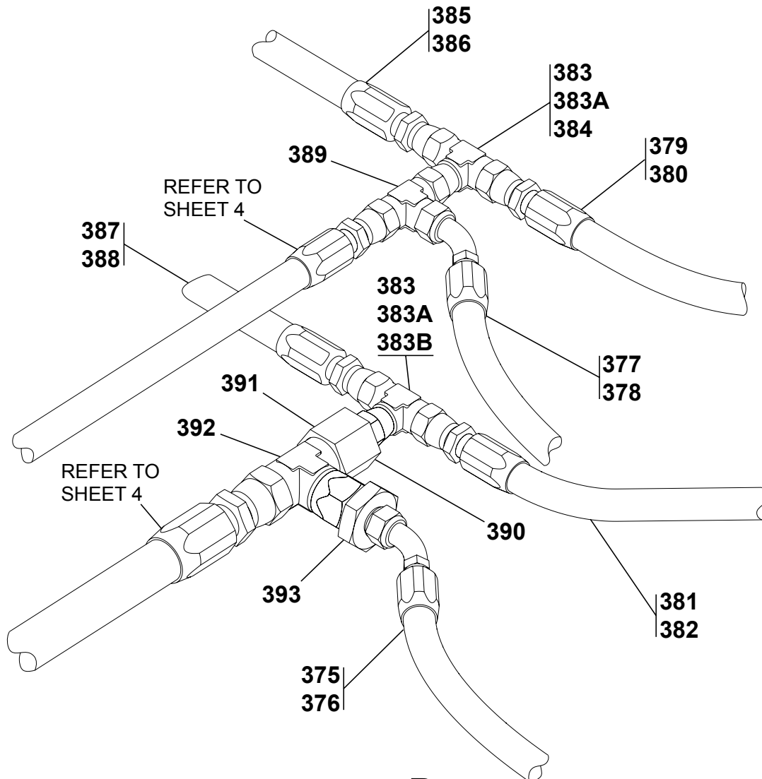
DETAIL B AIRPLANES 20800274 AND ON 208B0655 AND ON
