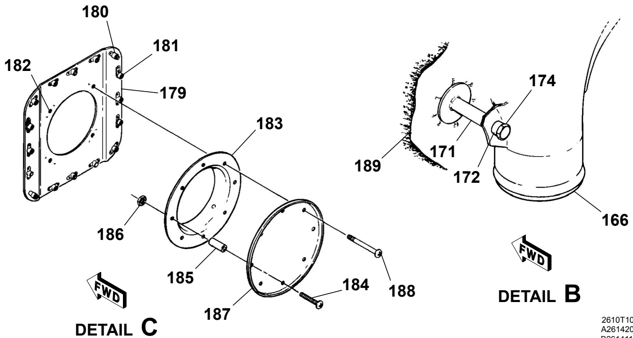
CABIN HEATING AND DEFROSTING SYSTEM Figure 01. (Sheet 3)
