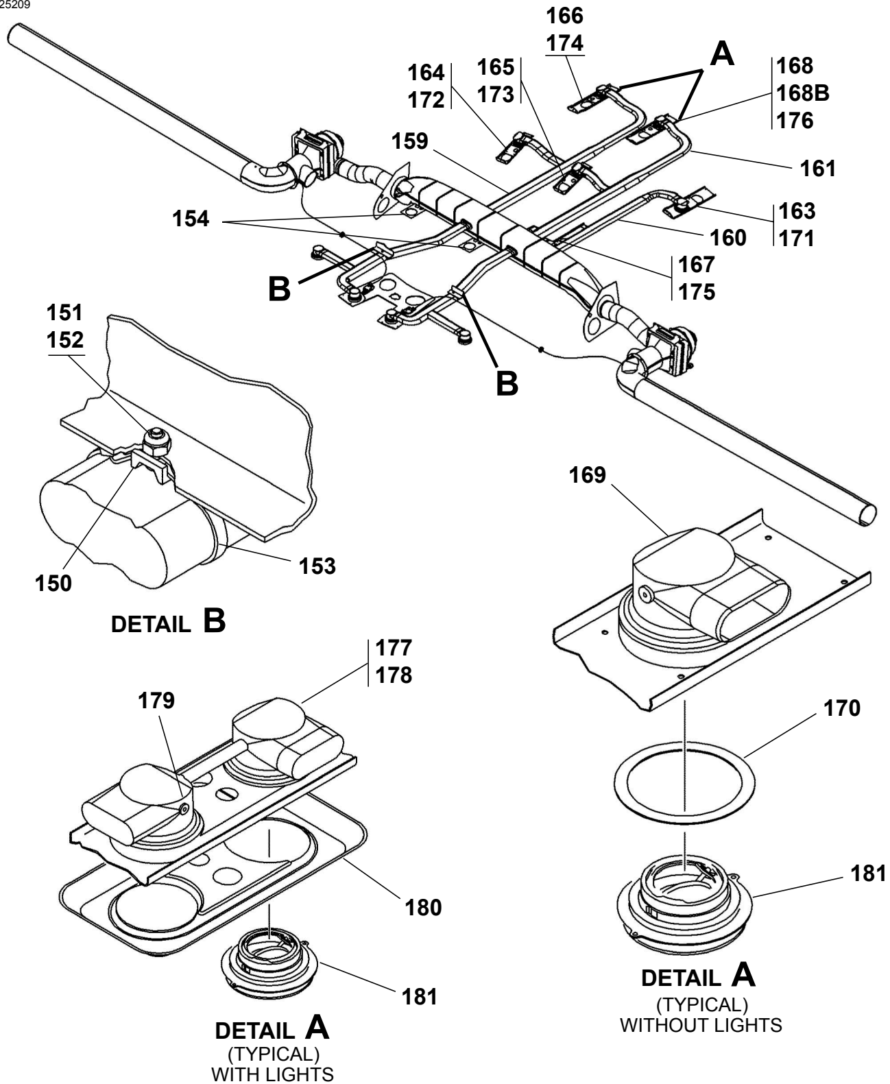
OVERHEAD VENTILATION SYSTEM WITH AIR CONDITIONING Figure 04. (Sheet 3)
