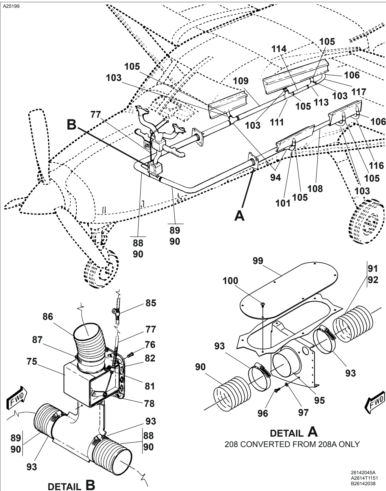
CABIN HEATING AND DEFROSTING SYSTEM Figure 01. (Sheet 2)
