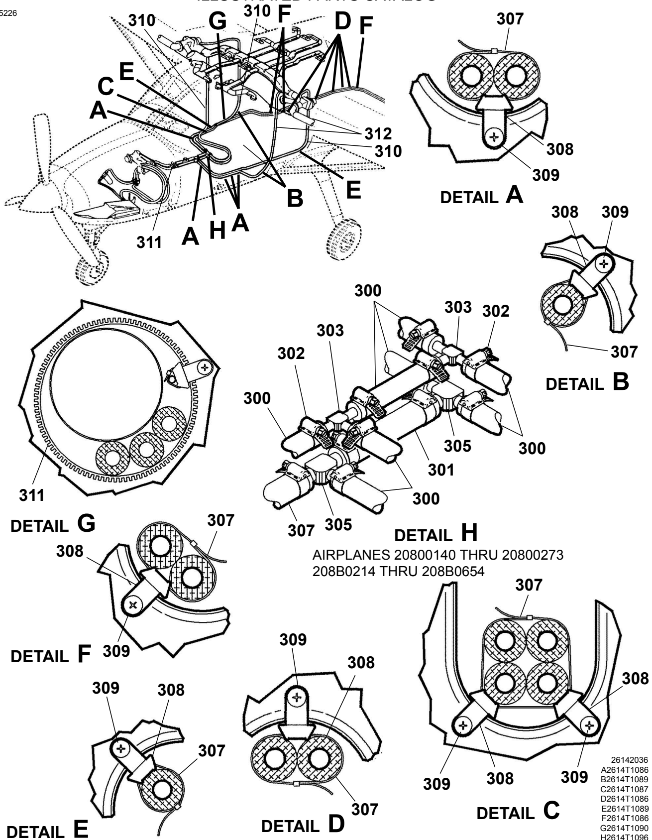
AIR CONDITIONING SYSTEM Figure 01. (Sheet 5)
