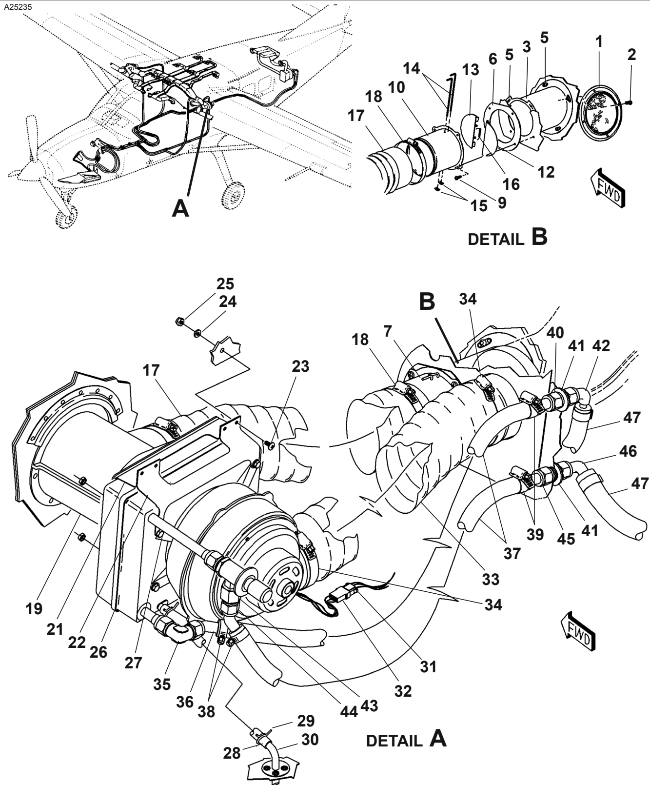
EVAPORATOR INSTALLATION - WING MOUNTED Figure 01. (Sheet 1)
