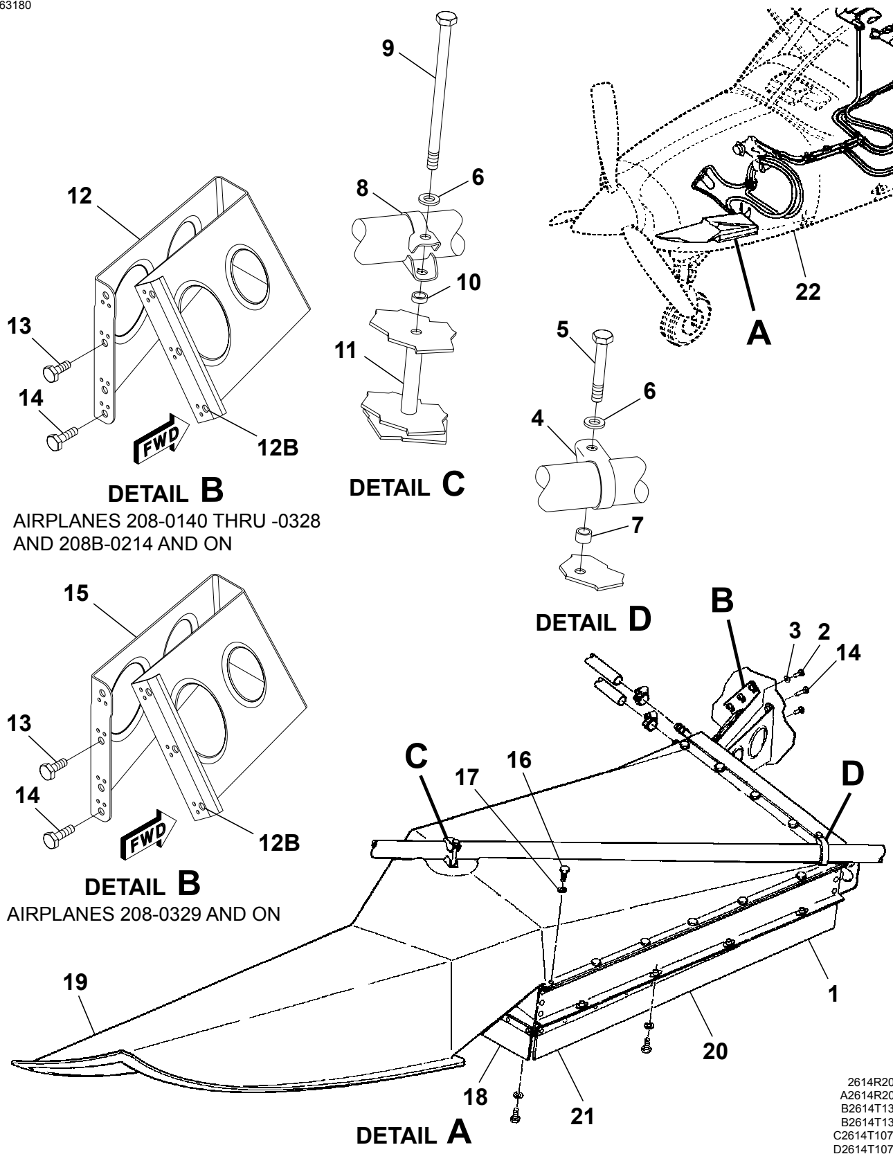
AIR CONDITIONER CONDENSER INSTALLATION Figure 01A. (Sheet 1)
