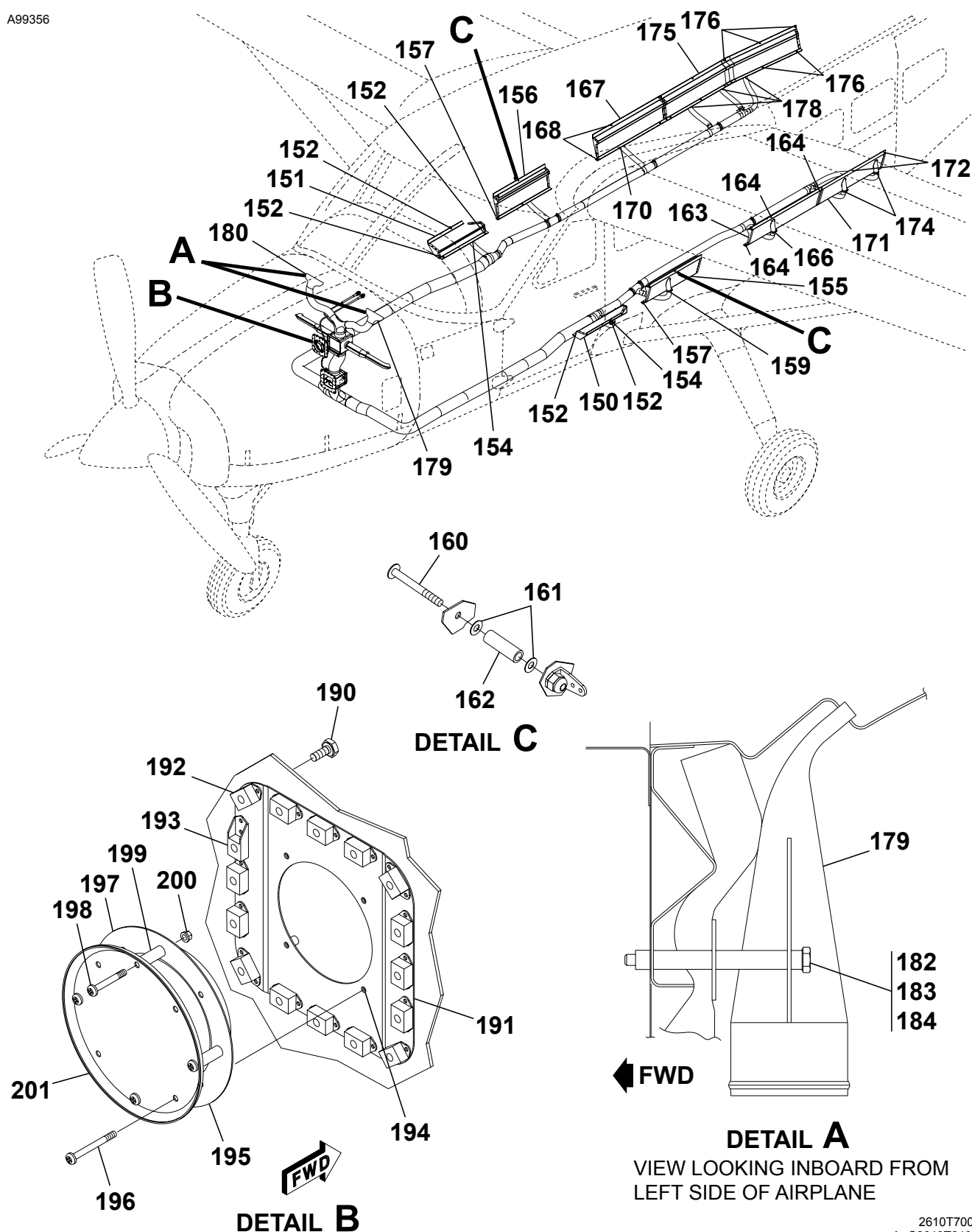
CABIN HEATING AND DEFROSTING SYSTEM - PASSENGER VERSION Figure 01A. (Sheet 3)
