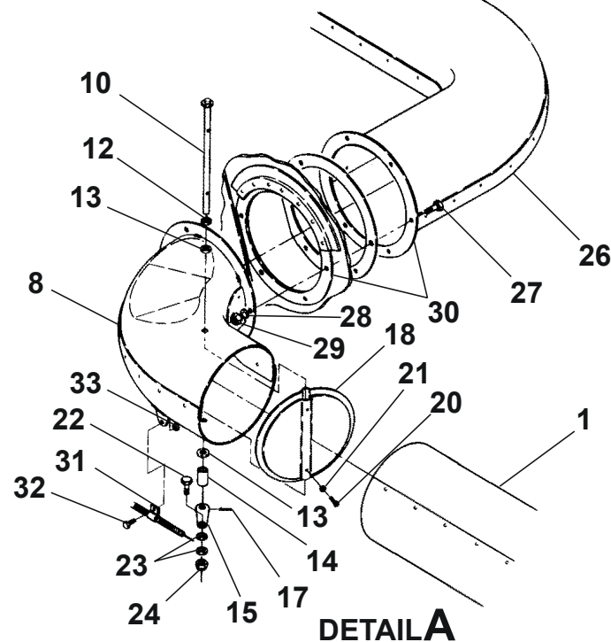
OVERHEAD VENTILATION SYSTEM - 208 Figure 01. (Sheet 1)
