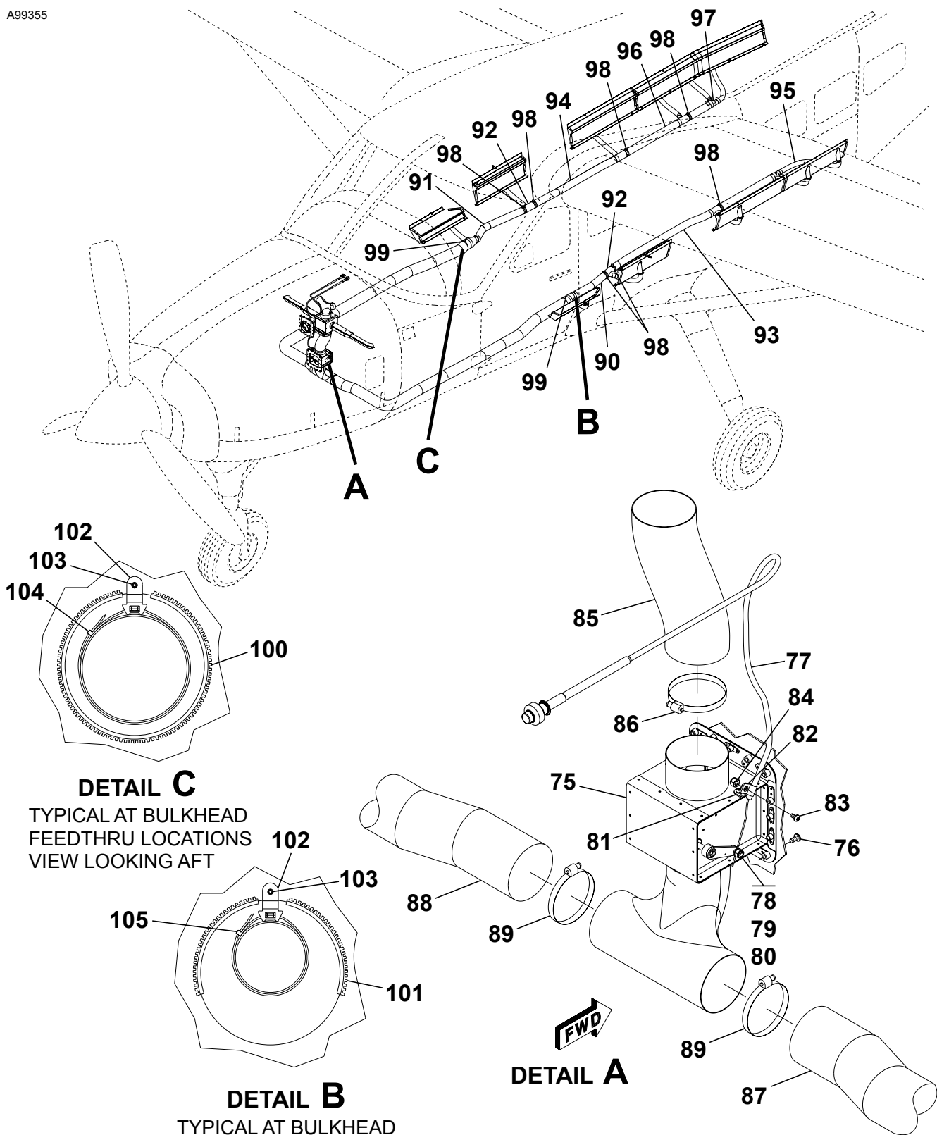
CABIN HEATING AND DEFROSTING SYSTEM - PASSENGER VERSION Figure 01A. (Sheet 2)
