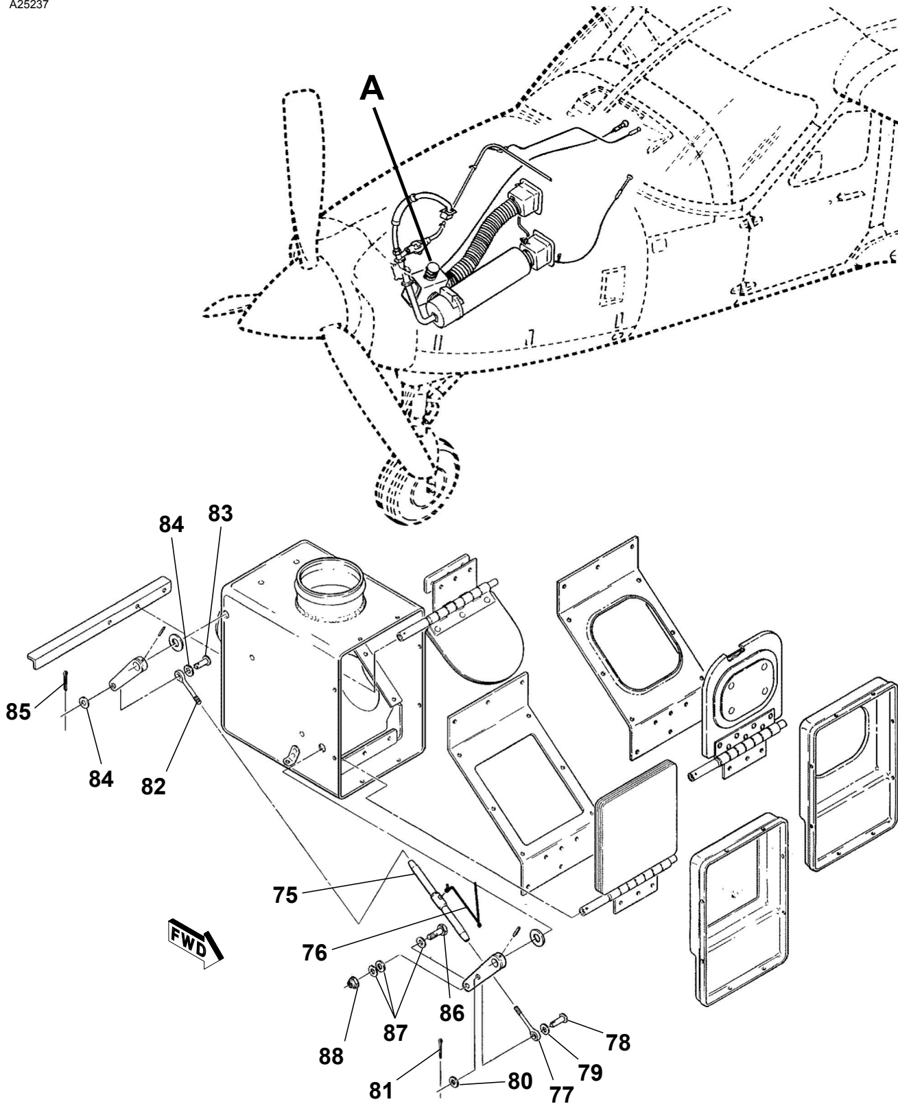
DIVERTER VALVE ASSEMBLIES - BLEED AIR Figure 01. (Sheet 2)
