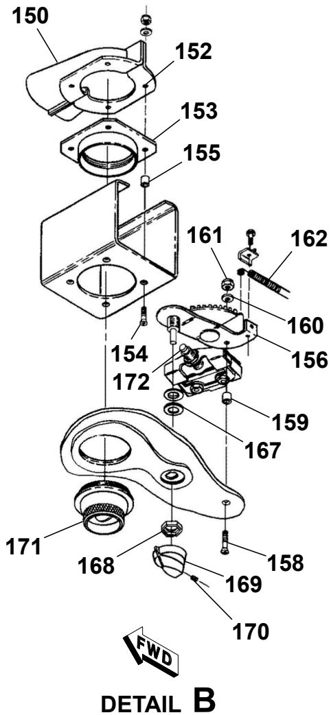
OVERHEAD VENTILATION SYSTEM WITHOUT AIR CONDITIONING Figure 01. (Sheet 3)
