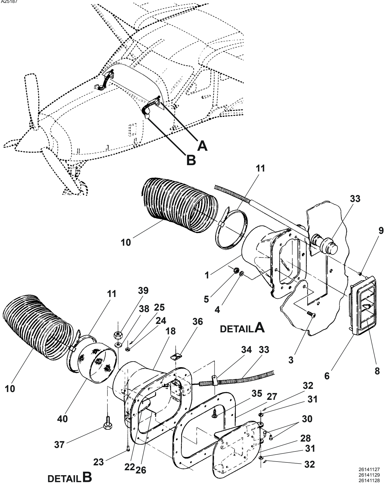
FORWARD VENTILATION SYSTEM Figure 01. (Sheet 1)
