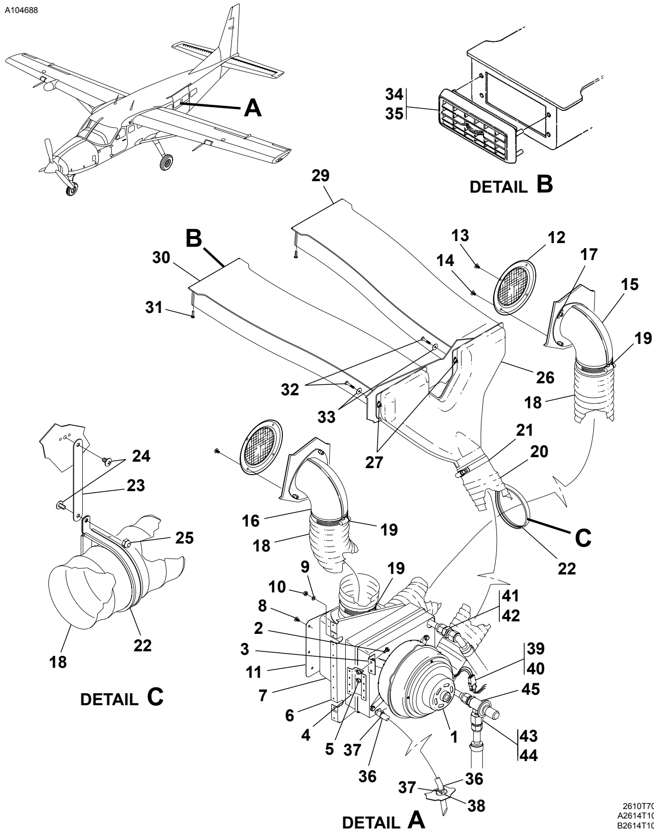
EVAPORATOR INSTALLATION - AFT MOUNTED Figure 01B. (Sheet 1)
