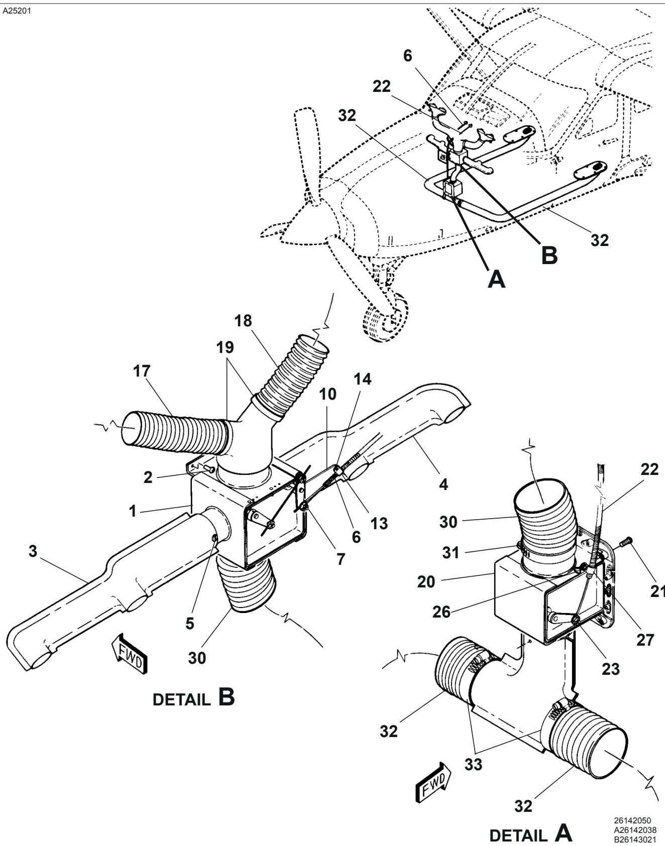
CABIN HEATING AND DEFROSTING SYSTEM Figure 01. (Sheet 1)
