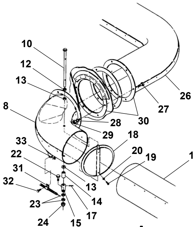
OVERHEAD VENTILATION SYSTEM Figure 01. (Sheet 1)
