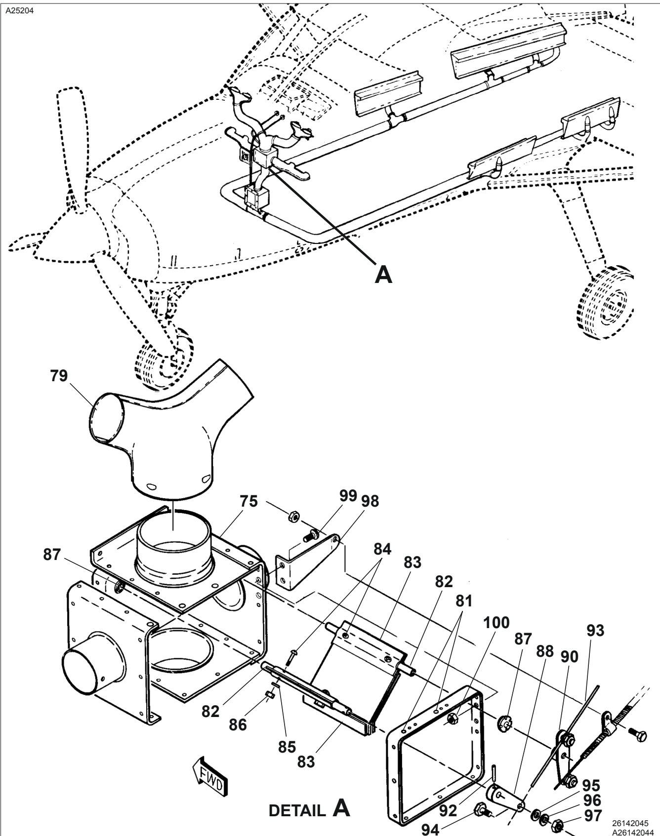
HEATER AND DEFROSTER VALVE ASSEMBLIES Figure 01. (Sheet 2)
