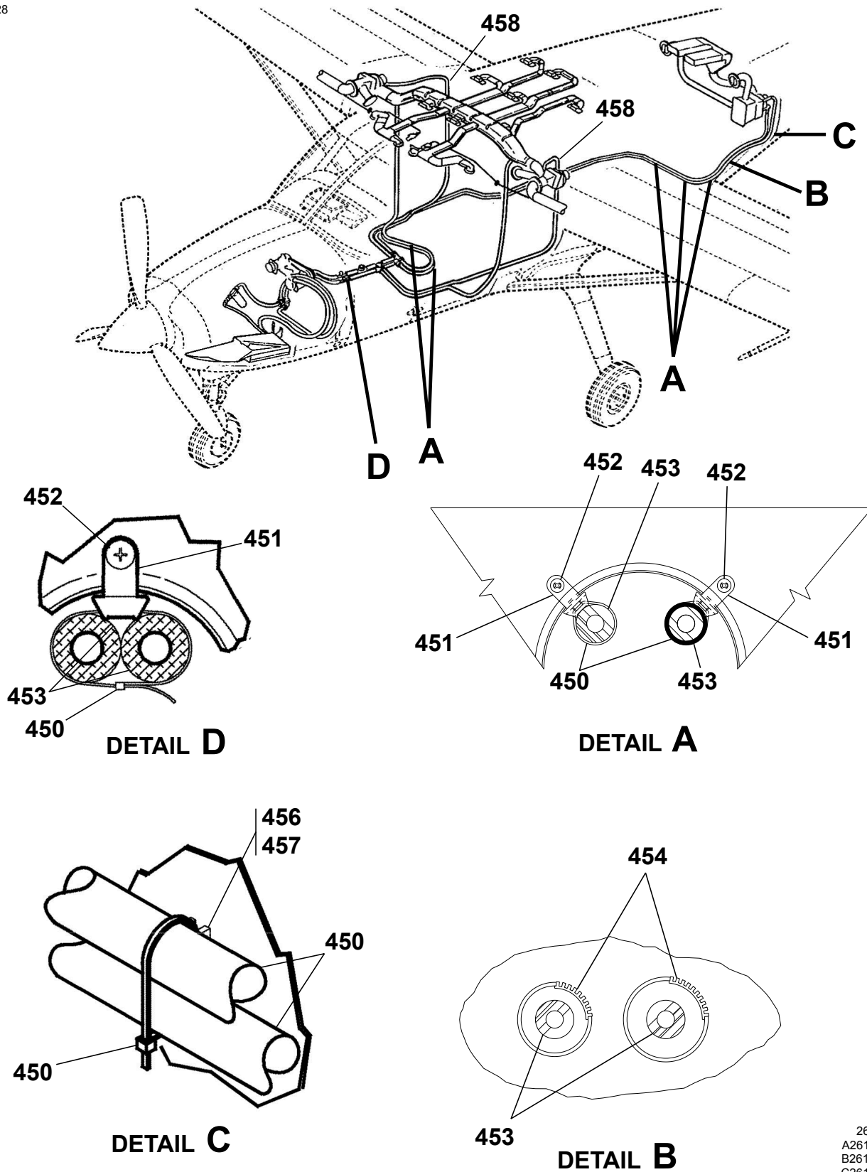
AIR CONDITIONING SYSTEM Figure 01. (Sheet 7)
