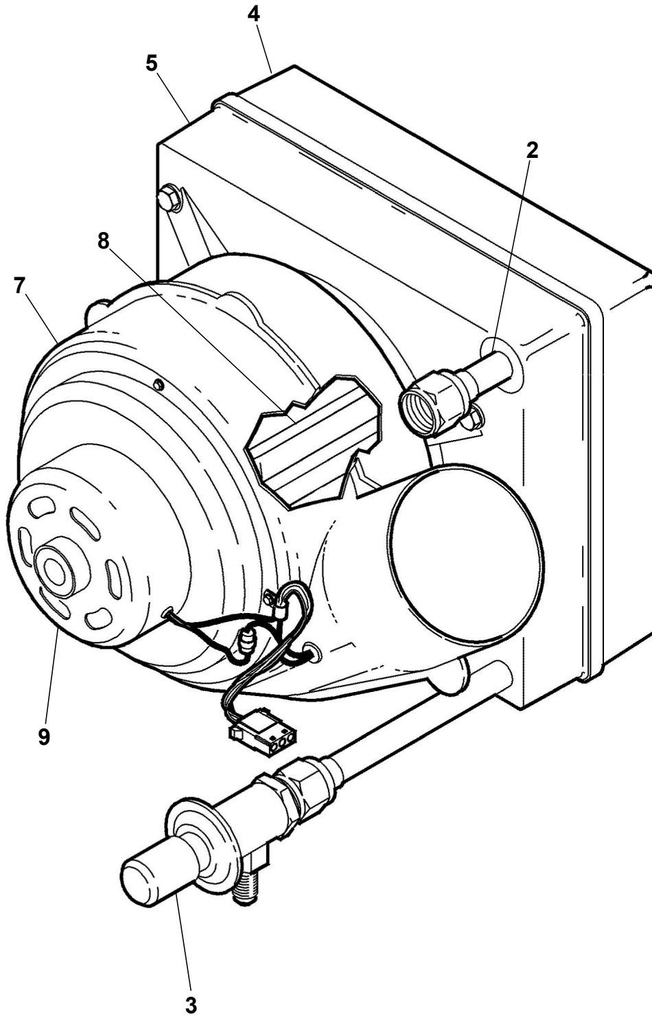
EVAPORATOR ASSEMBLY - AFT Figure 04. (Sheet 1)
