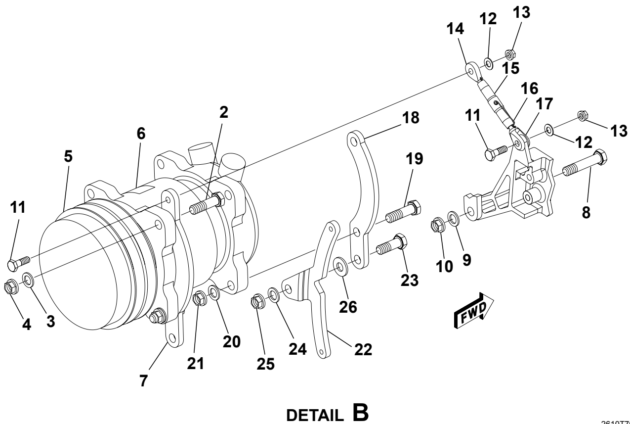
AIR CONDITIONER COMPRESSOR AND DRIVE UNIT INSTALLATION Figure 02A. (Sheet 1)
