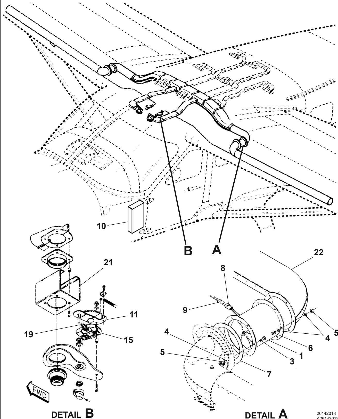
VENTILATION FAN INSTALLATION Figure 01. (Sheet 1)
