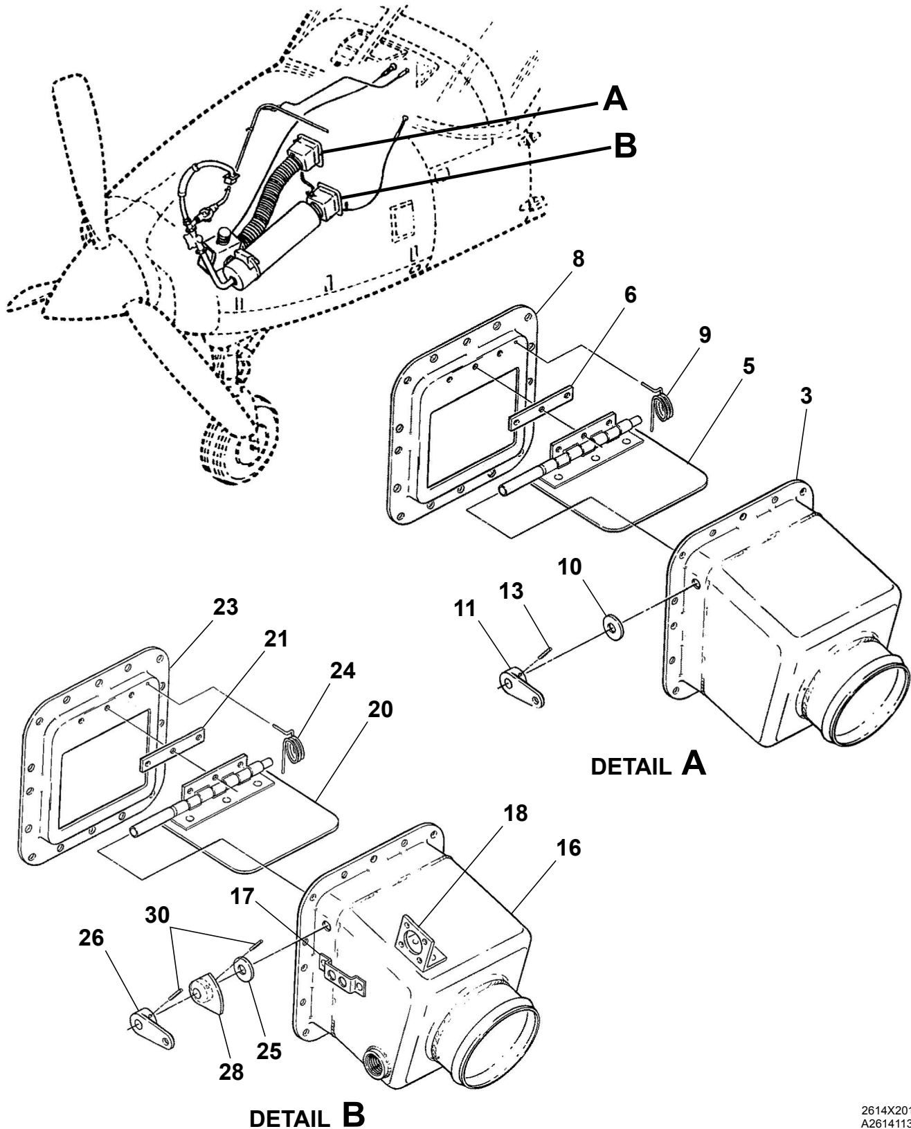
FIREWALL SHUTOFF VALVE ASSEMBLIES Figure 02. (Sheet 1)
