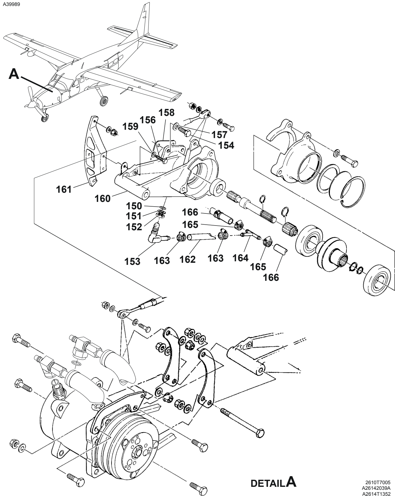
AIR CONDITIONER COMPRESSOR AND DRIVE UNIT INSTALLATION Figure 01. (Sheet 3)
