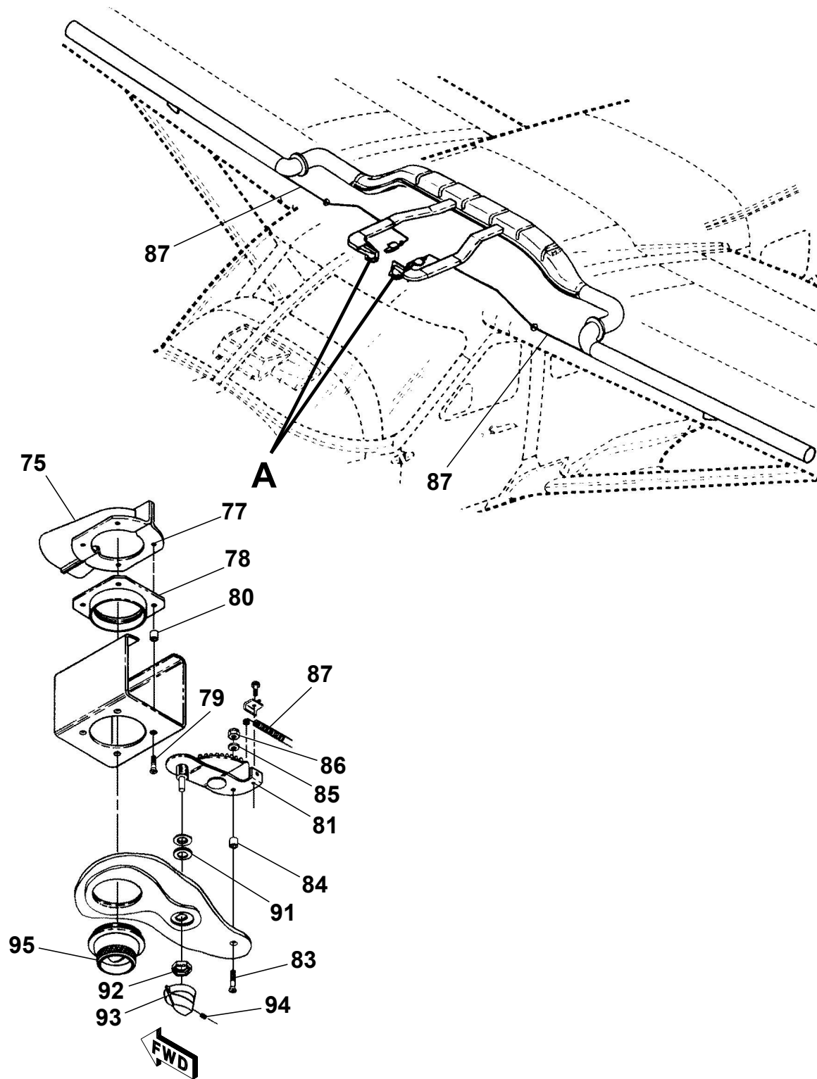
OVERHEAD VENTILATION SYSTEM Figure 01. (Sheet 2)
